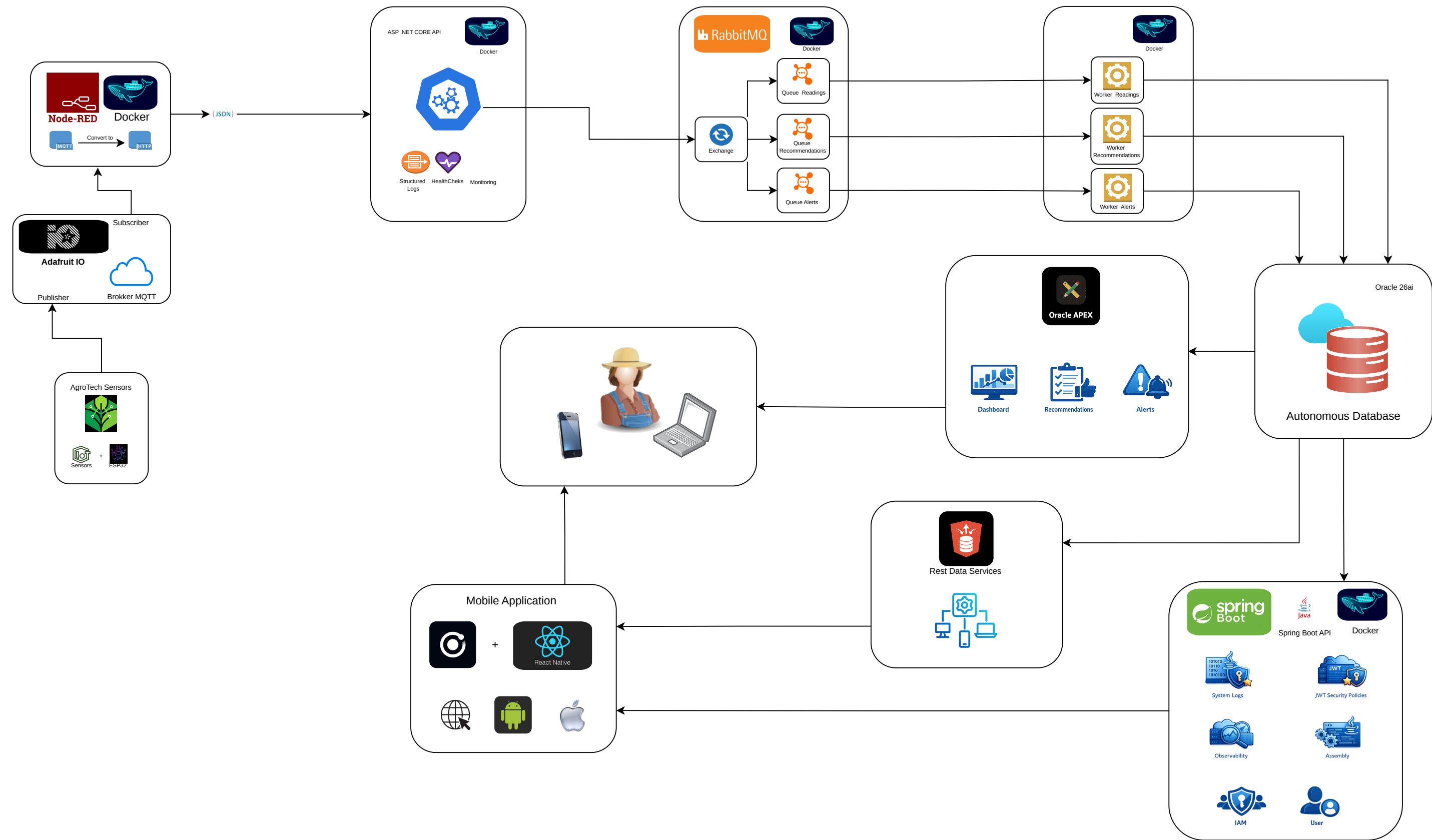
Flow 1 — IoT Monitoring, Processing and APEX Consumption
